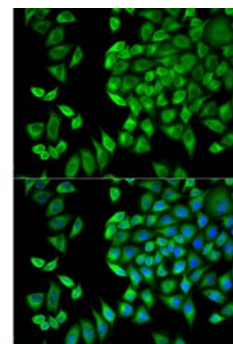
Fig. 2. Immunofluorescence analysis of HeLa cells using WNK1 antibody. Blue: DAPI for nuclear staining.
