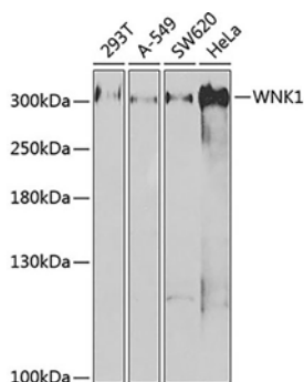
Fig. 1. Western blot analysis of extracts of various cell lines, using WNK1 antibody at 1:1000 dilution. Secondary antibody: HRP-labeled Goat Anti-Rabbit IgG(H+L) (A0208) at 1:1000 dilution. Lysates/proteins: 25µg per lane. Blocking buffer: QuickBlock™ Blocking Buffer (P0231). Detection: BeyoECL Star (P0018A). Exposure time:1s.
